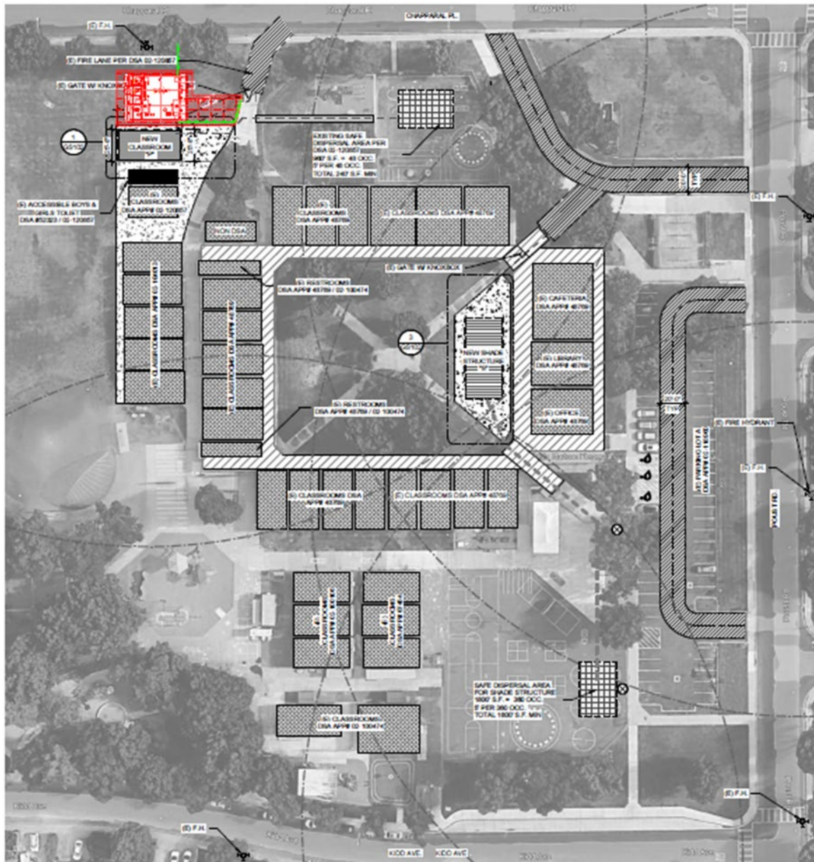
1 SITE PLAN - MARTONE ES 1" = 40'-0"
