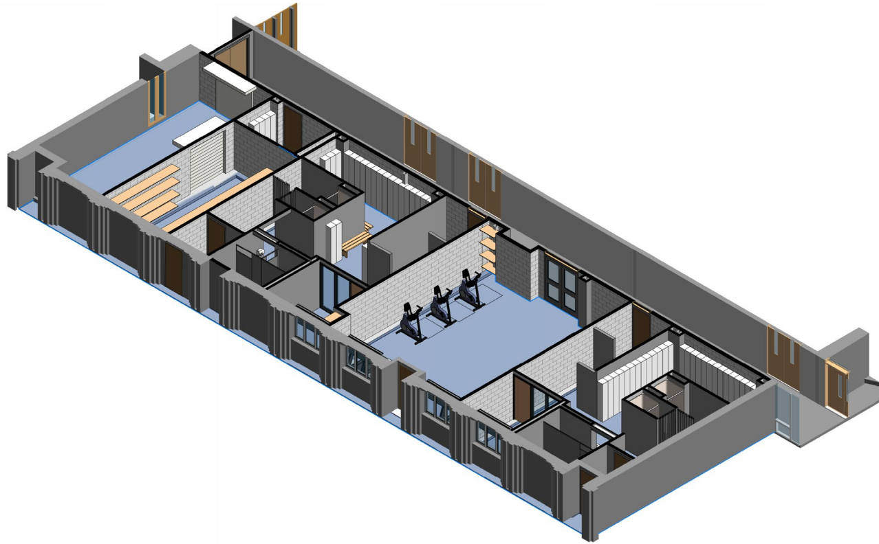
2 FITNESS SUITE - AXONOMETRIC
